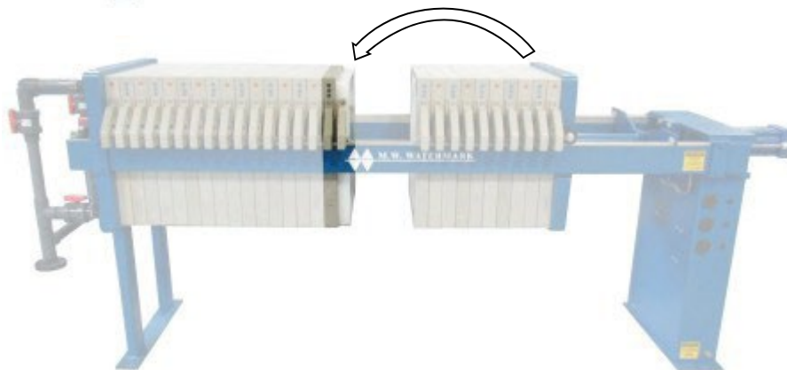
• Fig.2 - Tail and blanking plates moved forward in the plate stack
