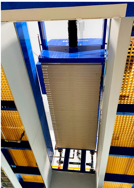
M.W. Watermark 630mm Filter Press with Discharge Chute, Elevated Platform and Bulk Bag
